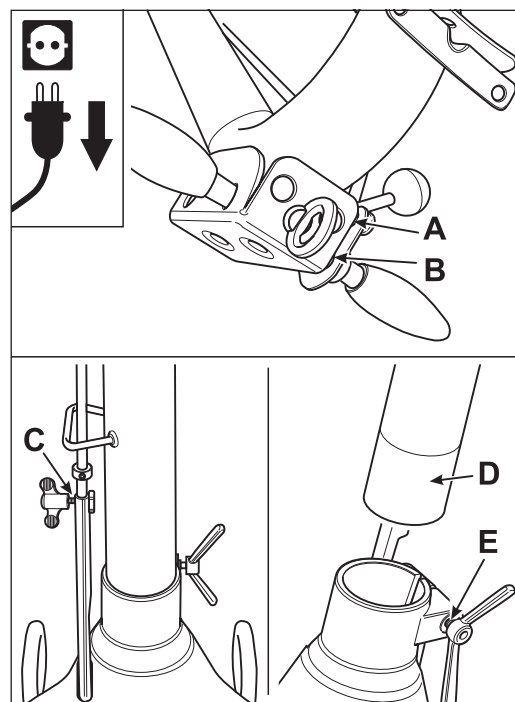
Fig. 65 Lubrication points which should be regularly oiled.
