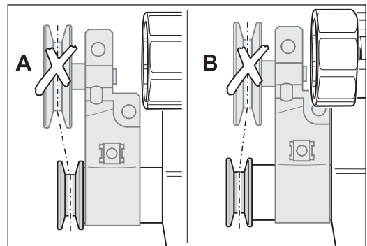
Fig. 103 Avoid position A and B of the belt tensioner! Otherwise the wearing of fan axle, pulleys and V-belt increase extensive!
